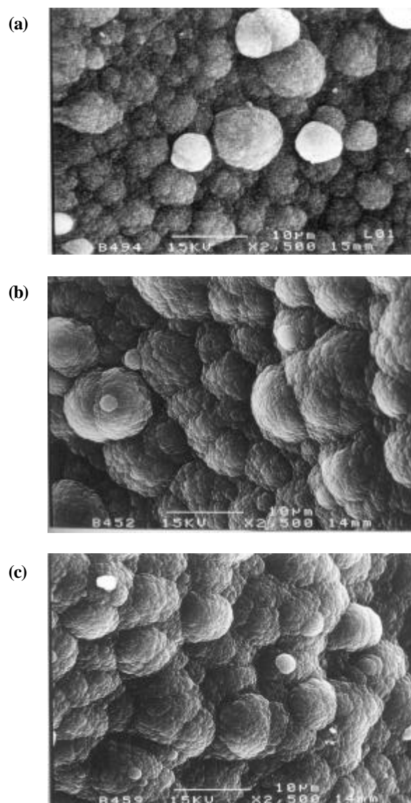
Figure 3. SEM micrographs (magnification 2500 times) of the films prepared at (a) 1.2°C, (b) 35.4°C and (c) 45.9°C.
